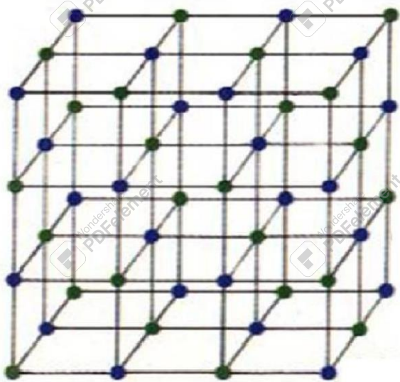
Crystalline three-dimensional-lattice-structure
